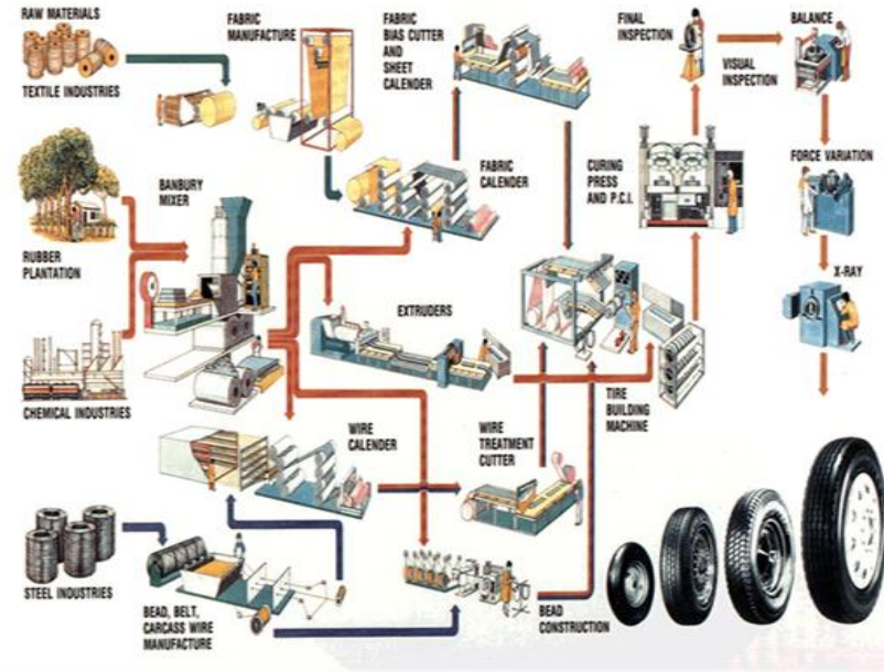
Source http://www.emt-india.net/process/tyre/tyre.htm
